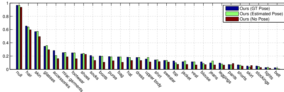
Fig. 7: Per class results for our model using Jaccard index metric on Fashionista v0.3.
